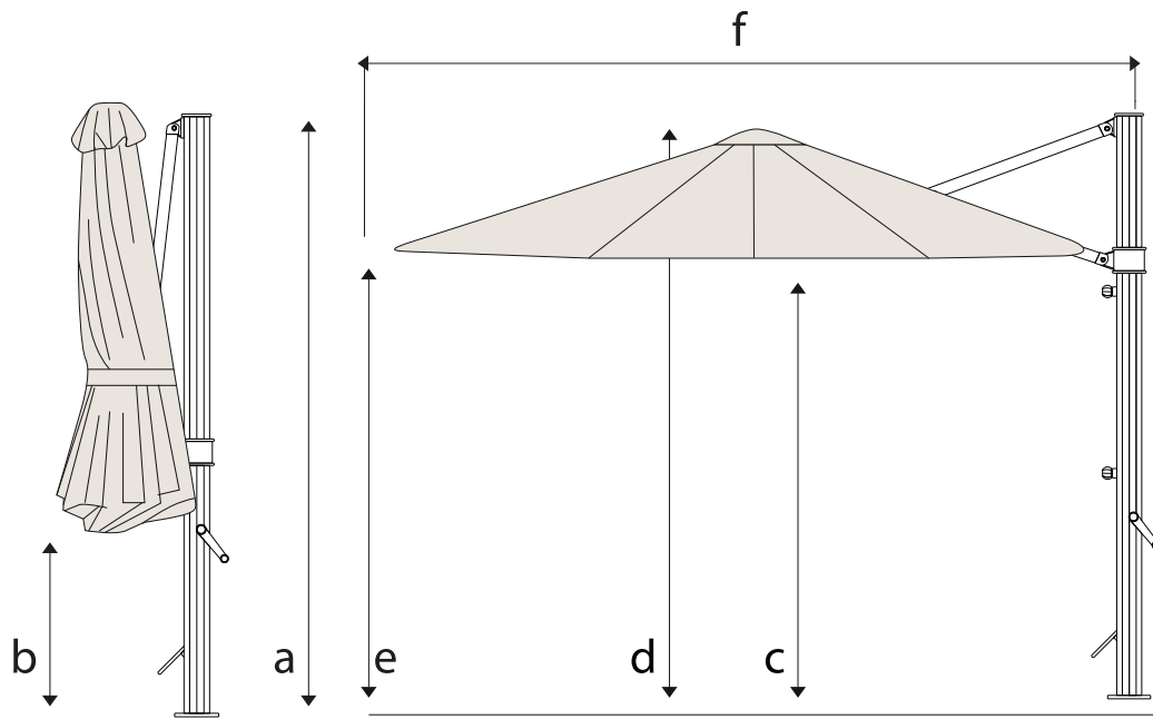
3.5m Octagonal
